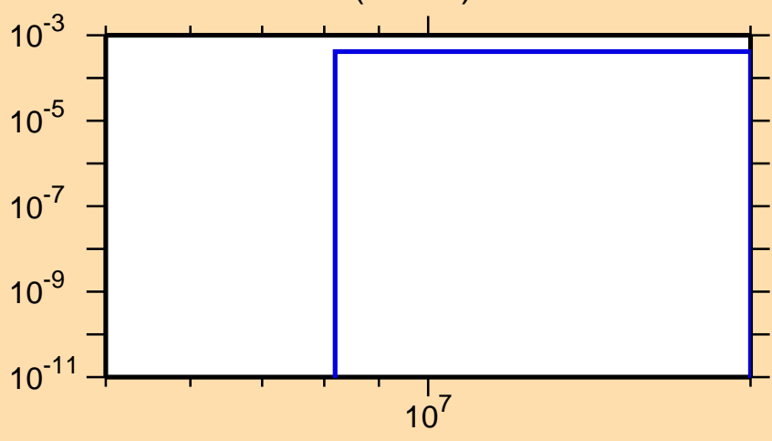
\sigma vs. E for ^{115}\text{I} (mt 45)
