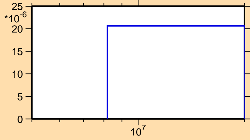
\sigma vs. E for ^{115}\text{I}(n,2np)
