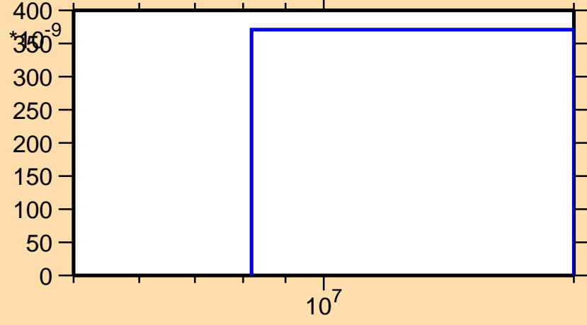
\sigma vs. E for ^{115}\text{I}(n,nd)
