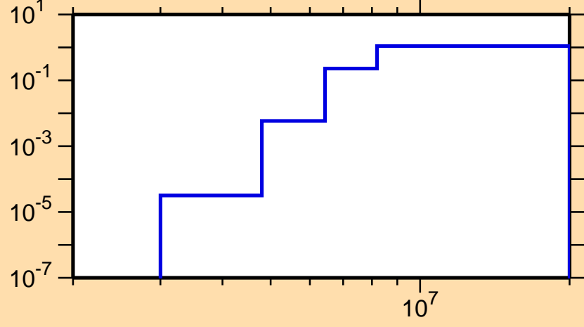
\sigma vs. E for ^{115}\text{I}(n,np)
