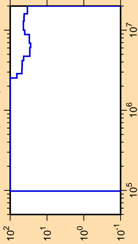
\Delta\sigma/\sigma vs. E for ^{116}\text{I}(n,\text{inel.})
