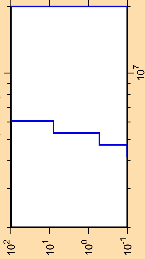
\Delta\sigma/\sigma vs. E for ^{116}\text{I}(n,\text{He3})
