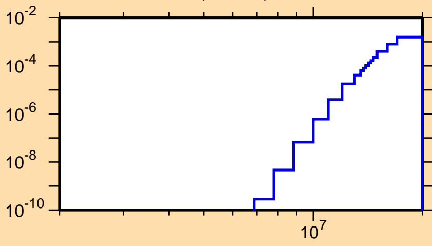
\sigma vs. E for ^{116}\text{I}(n,\text{He3})
