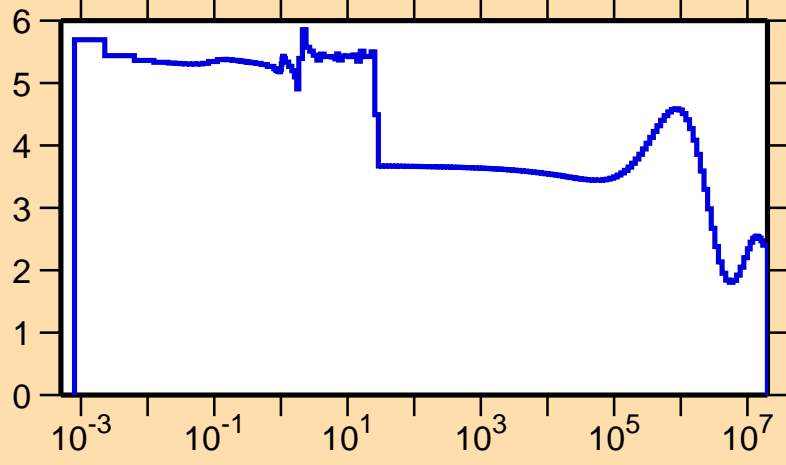
\sigma vs. E for ^{116}\text{I}(n,\text{el.})
