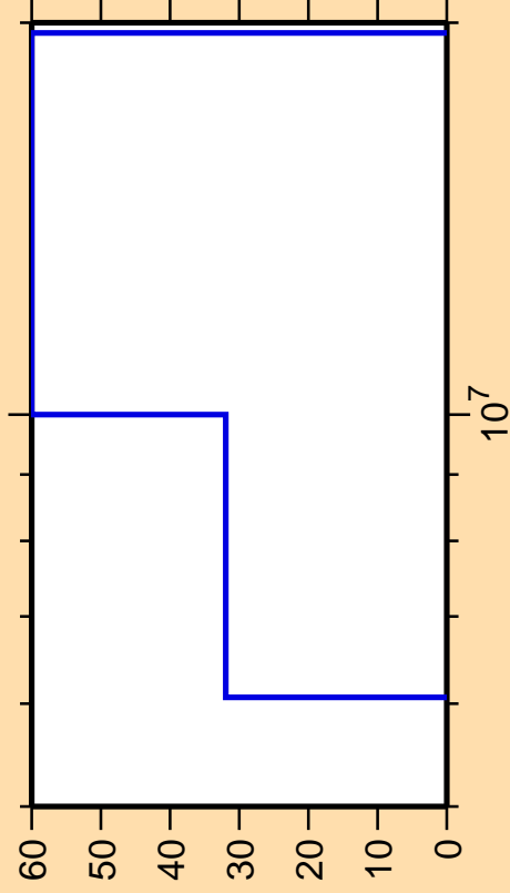
\Delta\sigma/\sigma vs. E for ^{116}\text{I} (mt 45)
