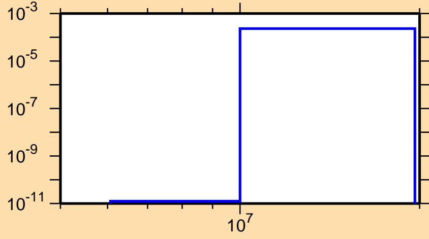
\sigma vs. E for ^{116}\text{I} (mt 45)
