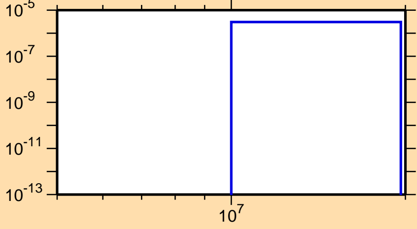
\sigma vs. E for ^{116}\text{I}(n,2n\alpha)
