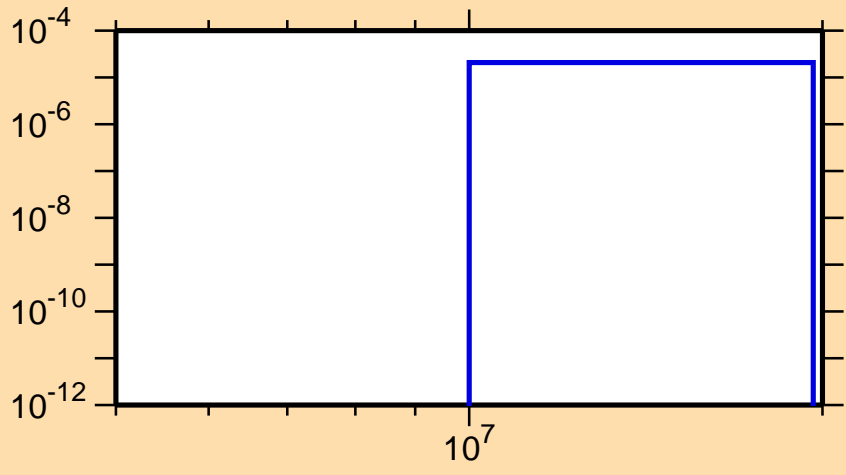
\sigma vs. E for ^{116}\text{I}(n,\text{pd})
