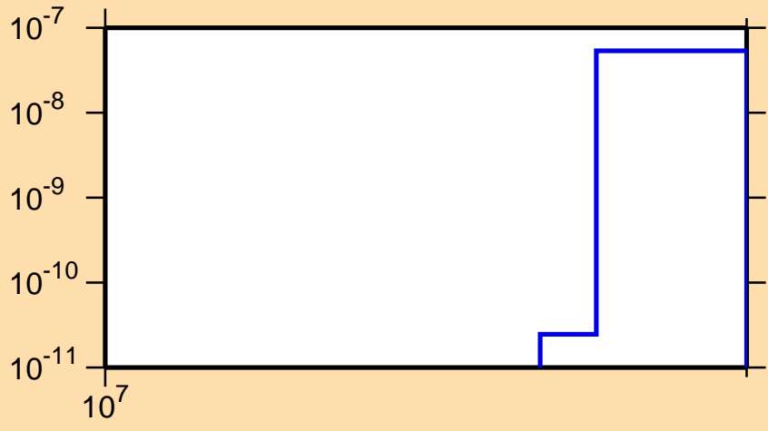
\sigma vs. E for ^{117}\text{I}(n,nt)
