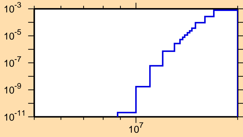
\sigma vs. E for ^{117}\text{I} (mt 45)
