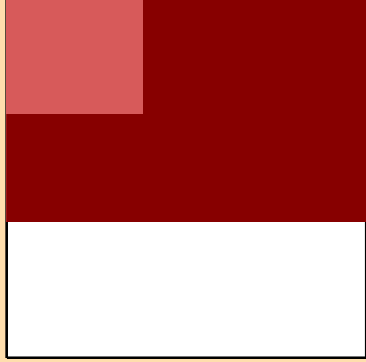
\Delta\sigma/\sigma vs. E for ^{117}\text{I}(n,\text{inel.})
