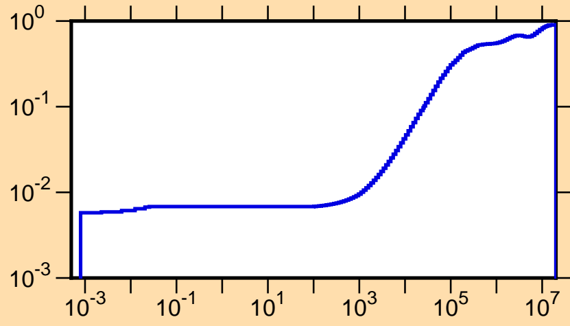
\mu vs. E for ^{118}\text{I}(\text{mt251})
