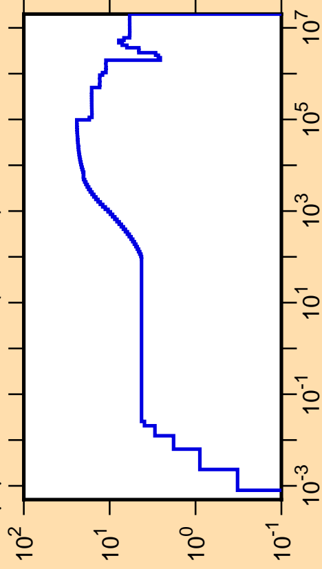
\Delta\mu/\mu vs. E for ^{118}\text{I}(\text{mt251})
