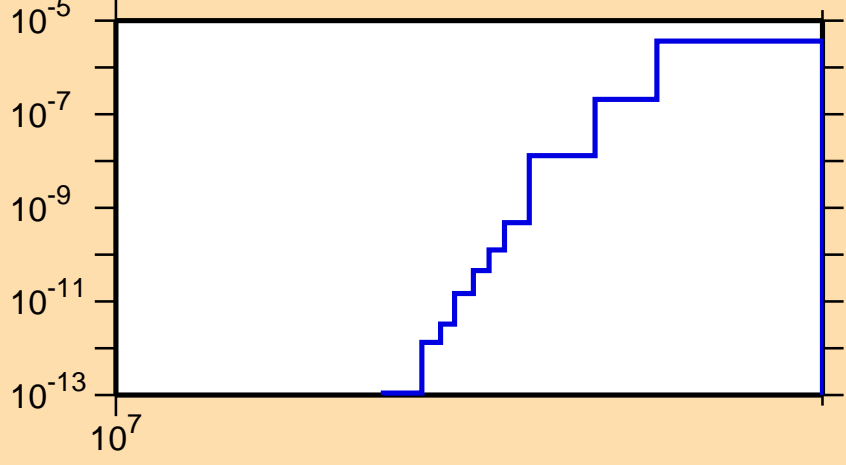
\sigma vs. E for ^{118}\text{I}(n,pt)
