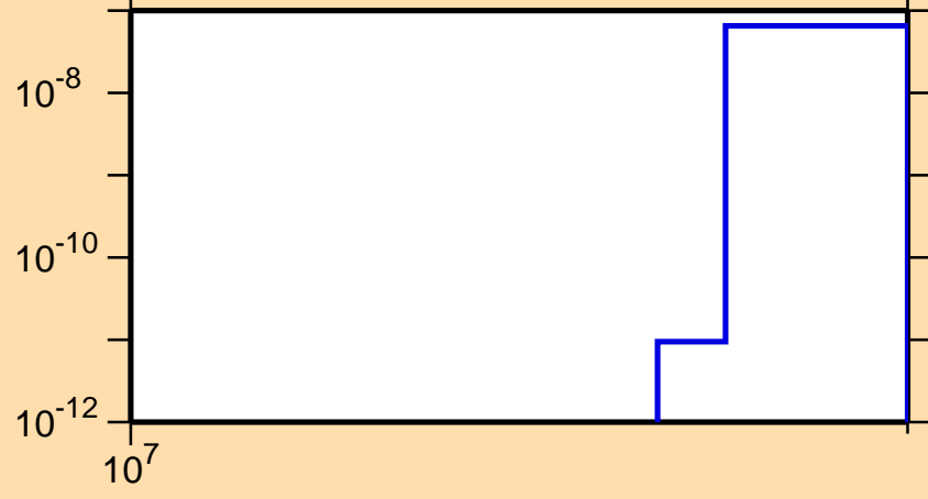
\sigma vs. E for ^{118}\text{I}(n,nt)
