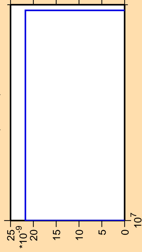
\Delta\sigma/\sigma vs. E for ^{118}\text{I}(n,3n\alpha)
