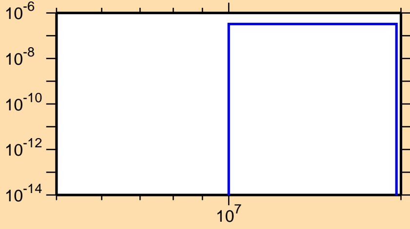
\sigma vs. E for ^{118}\text{I}(n,\text{pd})
