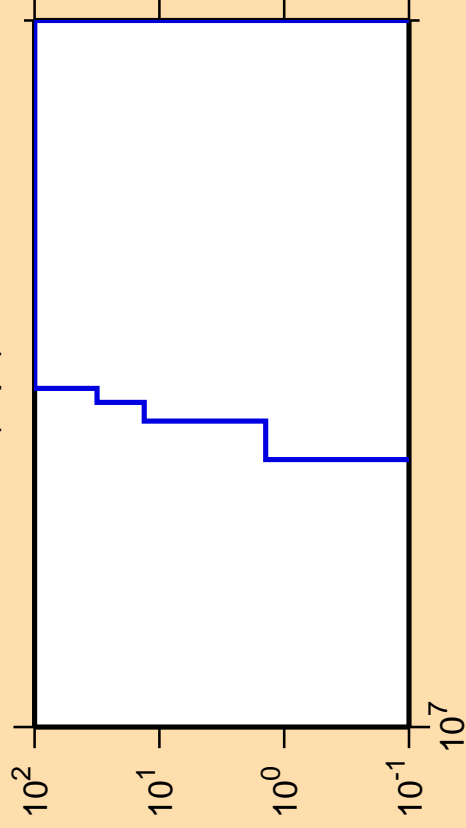
\Delta\sigma/\sigma vs. E for ^{118}\text{I}(n,pt)
