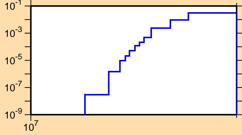
\sigma vs. E for ^{118}\text{I}(n,2np)
