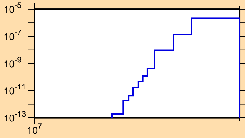
\sigma vs. E for ^{118}\text{I}(n,pt)
