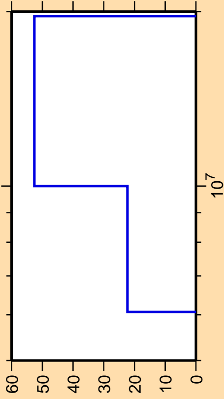
\Delta\sigma/\sigma vs. E for ^{118}\text{I}(n,\gamma)
