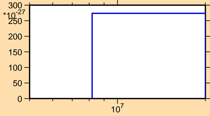
\sigma vs. E for ^{118}\text{I} (mt 11)
