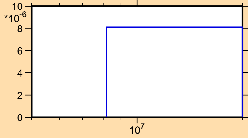
\sigma vs. E for ^{118}\text{I}(n,\text{nd})
