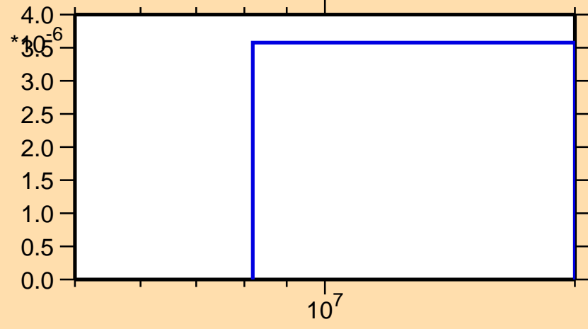
\sigma vs. E for ^{118}\text{I} (mt 45)
