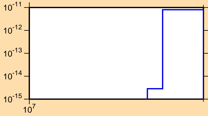
\sigma vs. E for ^{119}\text{I} (mt 34)
