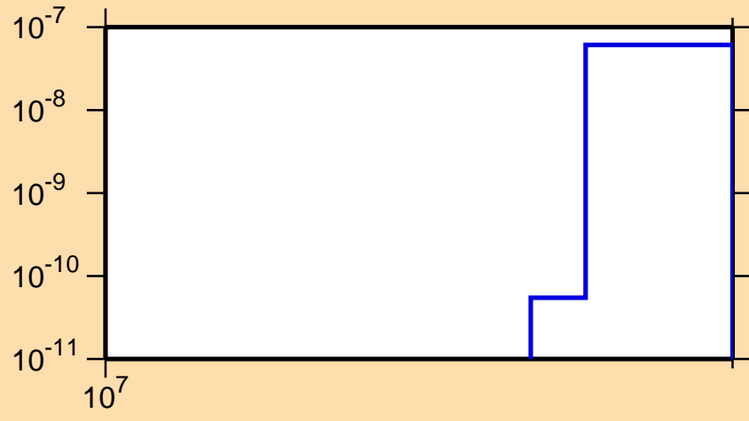
\sigma vs. E for ^{119}\text{I}(n,nt)
