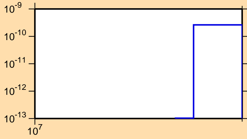
\sigma vs. E for ^{119}\text{I}(n,\text{pt})
