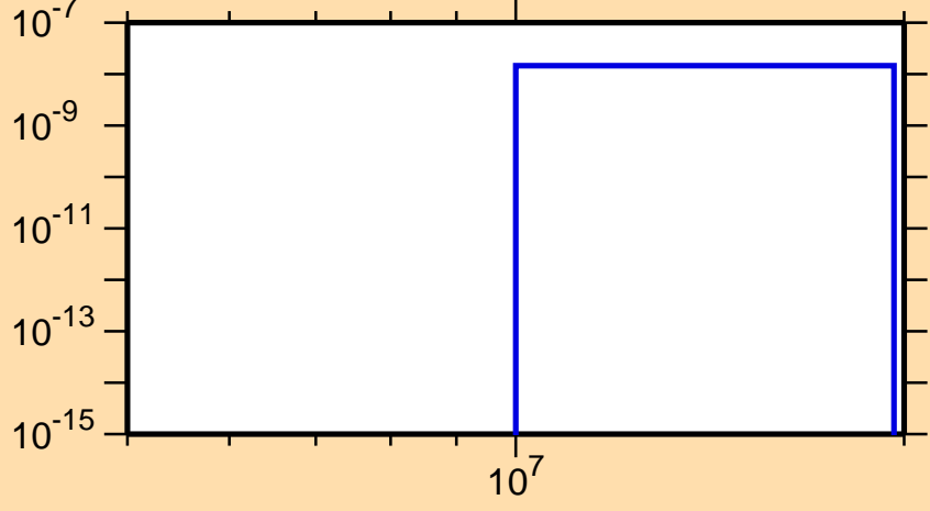
\sigma vs. E for ^{119}\text{I}(\text{mt117})
