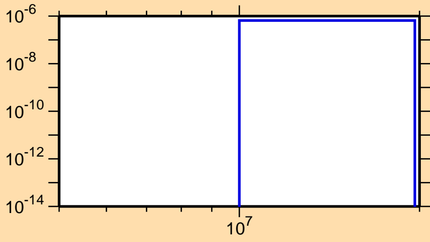
\sigma vs. E for ^{119}\text{I} (mt 45)
