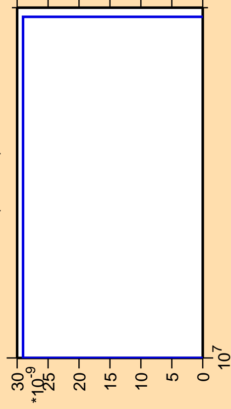
\Delta\sigma/\sigma vs. E for ^{119}\text{I}(n,3n\alpha)
