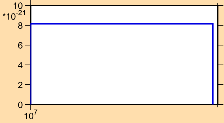
\sigma vs. E for ^{119}\text{I}(n,3n\alpha)
