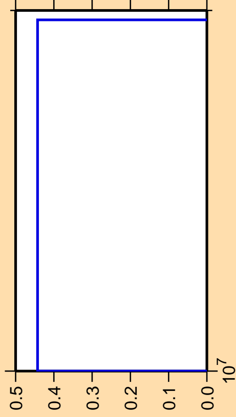
\Delta\sigma/\sigma vs. E for ^{119}\text{I} (mt 34)
