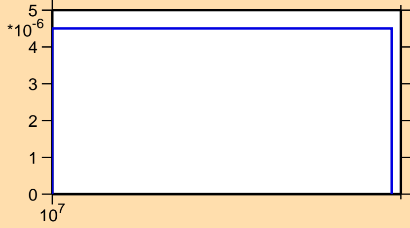
\sigma vs. E for ^{119}\text{I}(n,2np)
