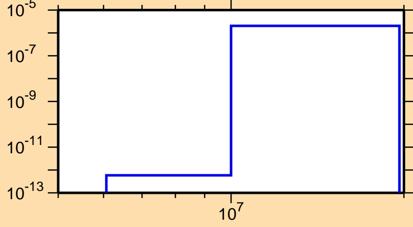
\sigma vs. E for ^{119}\text{I}(n,\text{He3})
