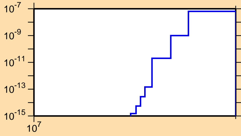
\sigma vs. E for ^{120}\text{I}(n,pt)
