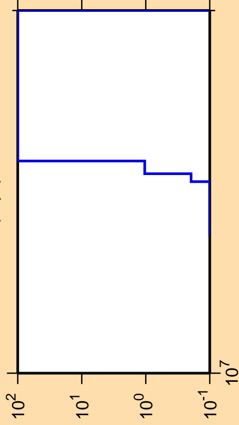
\Delta\sigma/\sigma vs. E for ^{120}\text{I}(n,pt)
