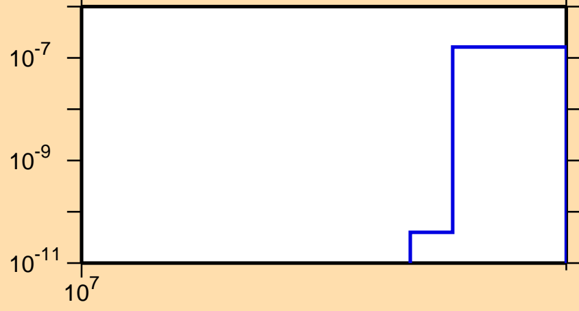
\sigma vs. E for ^{120}\text{I}(n,nt)
