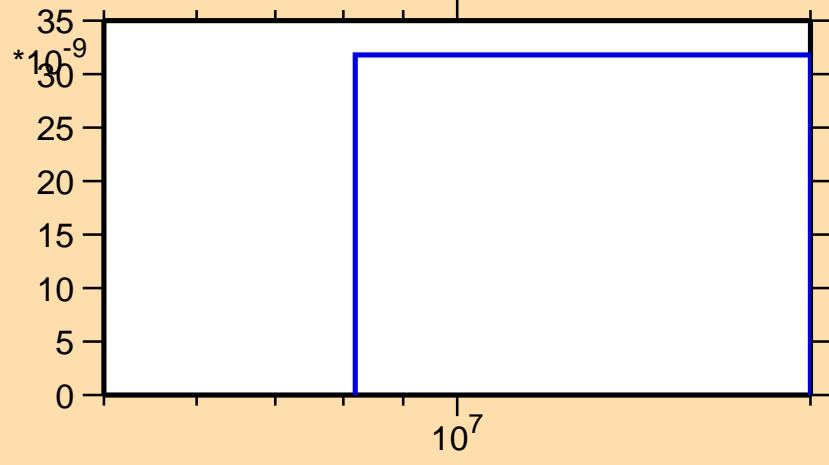
\sigma vs. E for ^{120}\text{I} (mt 45)
