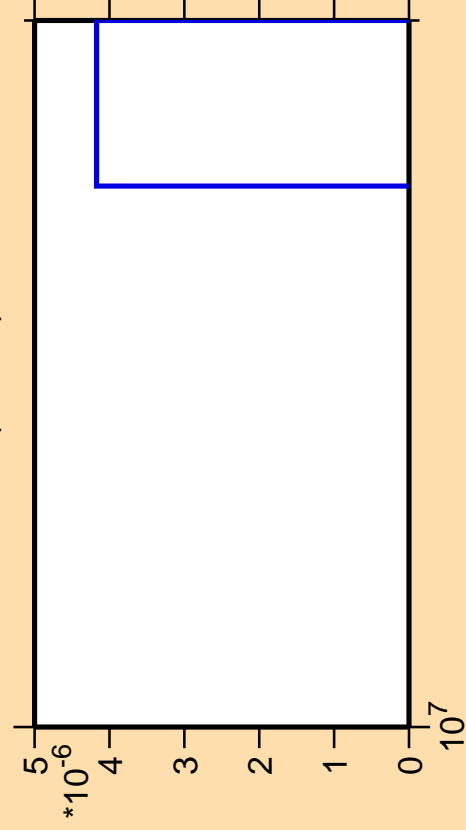
\Delta\sigma/\sigma vs. E for ^{120}\text{I} (mt 11)
