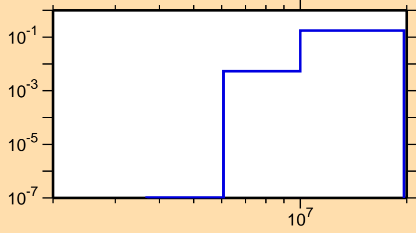
\sigma vs. E for ^{120}\text{I}(n,np)
