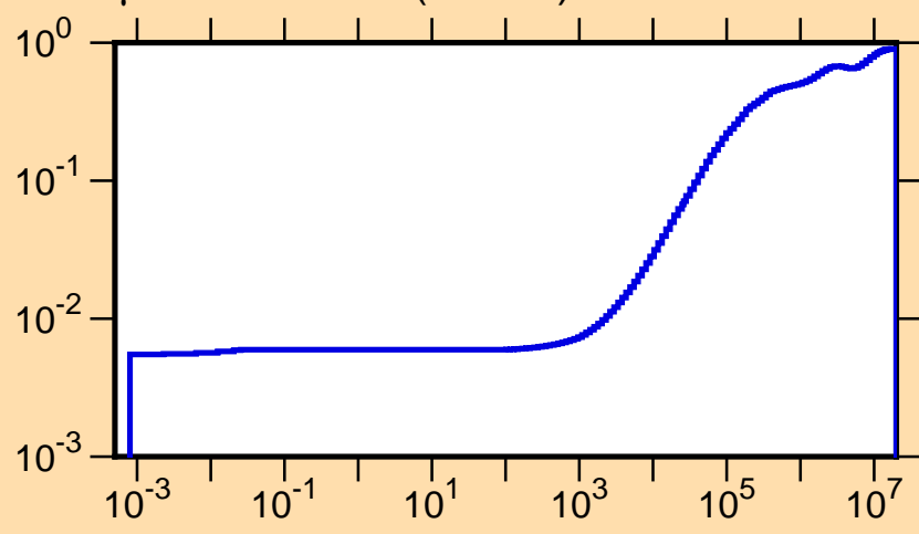
\mu vs. E for ^{123}\text{I}(\text{mt251})
