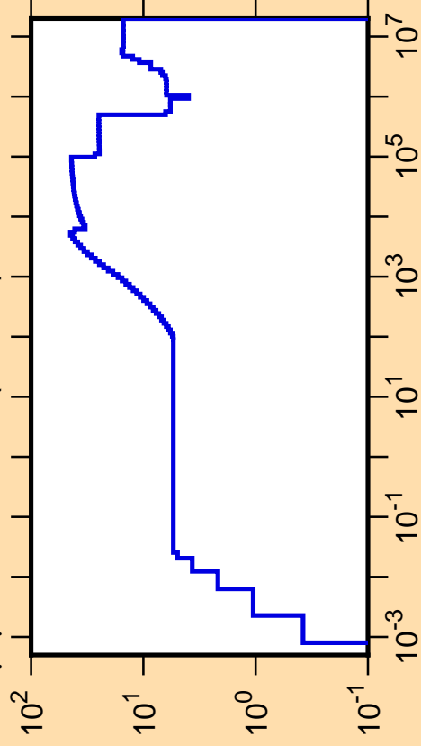
\Delta\mu/\mu vs. E for ^{123}\text{I}(\text{mt251})
