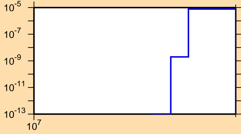
\sigma vs. E for ^{123}\text{I}(n,2np)
