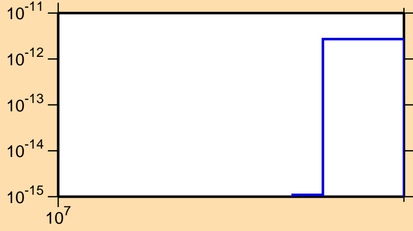
\sigma vs. E for ^{124}\text{I}(n,\text{pd})
