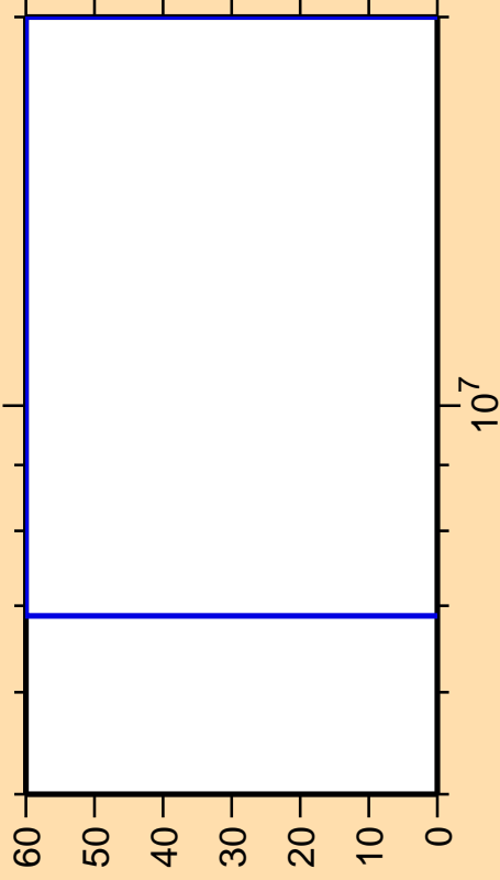
\Delta\sigma/\sigma vs. E for ^{124}\text{I}(n,\alpha)
