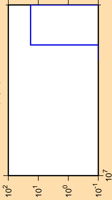
\Delta\sigma/\sigma vs. E for ^{124}\text{I}(n,\text{pd})
