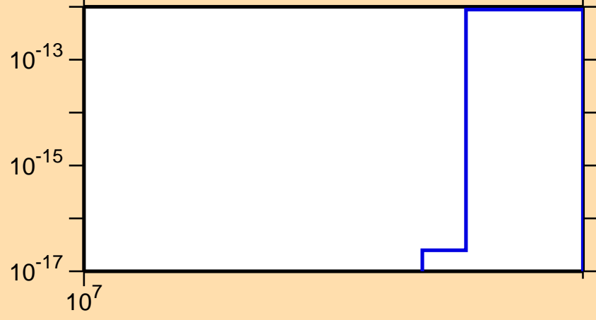
\sigma vs. E for ^{124}\text{I} (mt 34)
