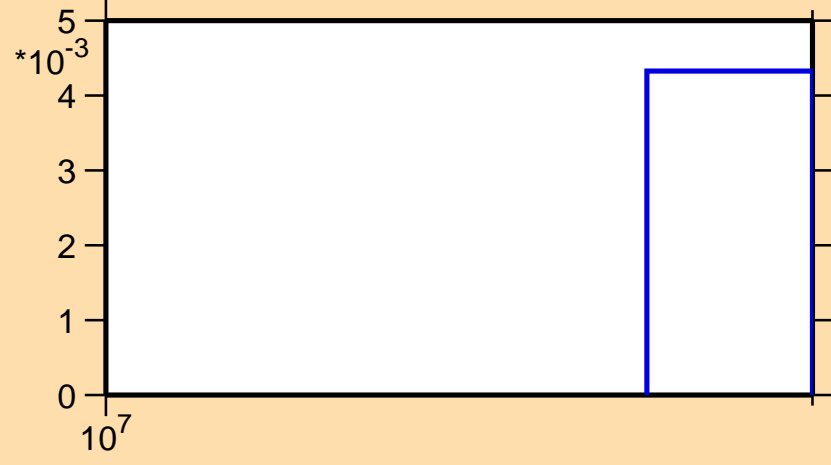
\sigma vs. E for ^{124}\text{I}(n,3n)
