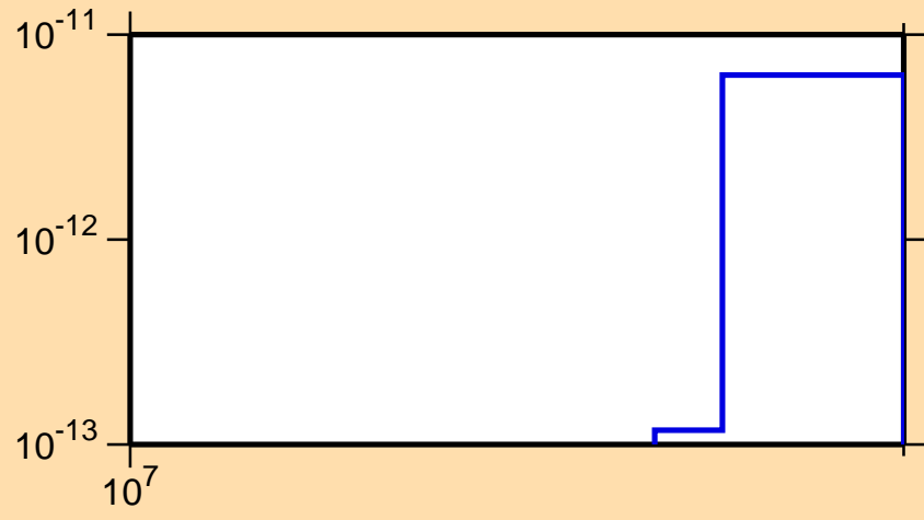
\sigma vs. E for ^{124}\text{I} (mt 45)
