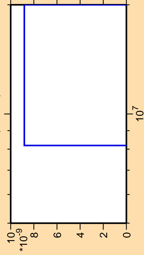
\Delta\sigma/\sigma vs. E for ^{124}\text{I}(n,3n\alpha)
