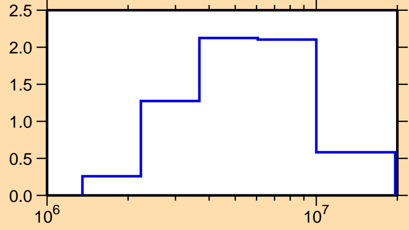
\sigma vs. E for ^{125}\text{I}(n,n\text{cont.})
