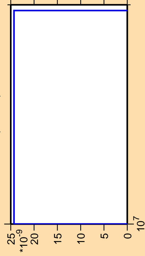
\Delta\sigma/\sigma vs. E for ^{125}\text{I}(n,3n\alpha)
