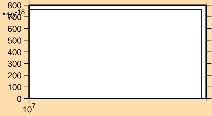
\sigma vs. E for ^{125}\text{I}(n,\text{pd})
