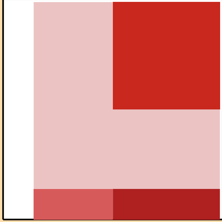
\Delta\sigma/\sigma vs. E for ^{125}\text{I}(n,2n)
