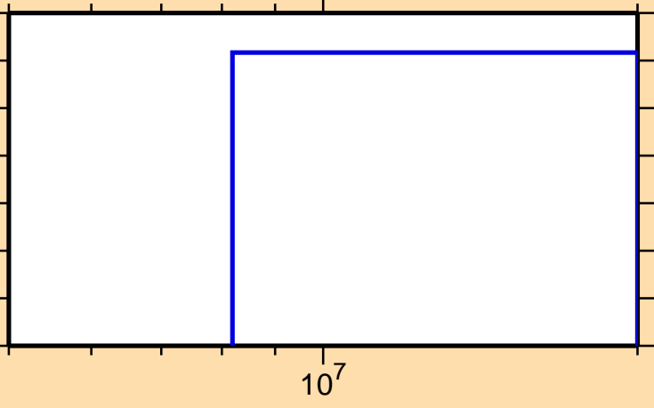
\sigma vs. E for ^{125}\text{I}(n,\text{He3})
