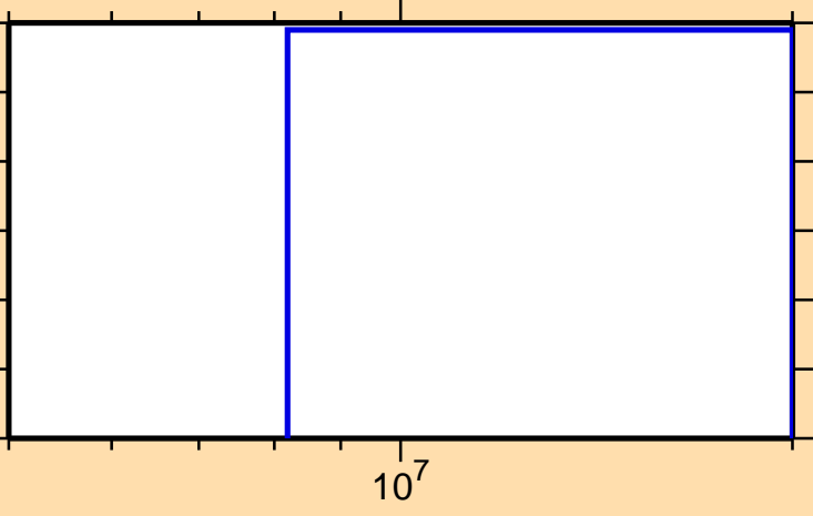
\sigma vs. E for ^{125}\text{I}(n,nt)
