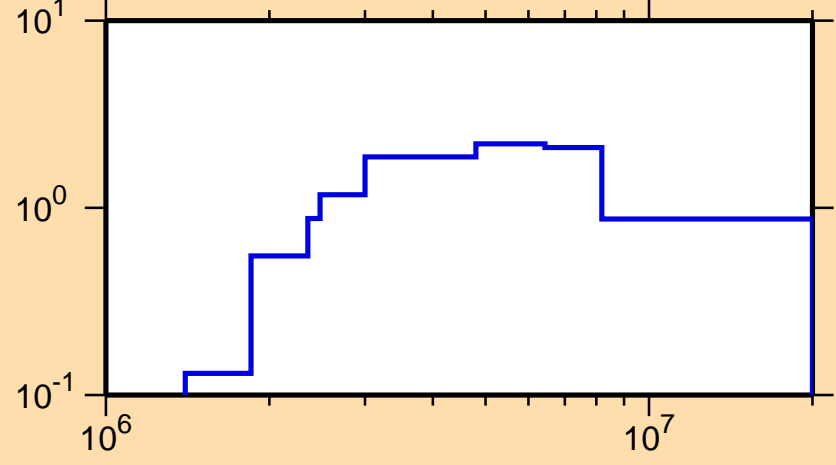
\sigma vs. E for ^{125}\text{I}(n,n\text{cont.})
