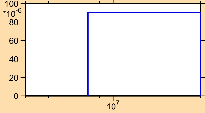
\sigma vs. E for ^{125}\text{I}(n,3n)
