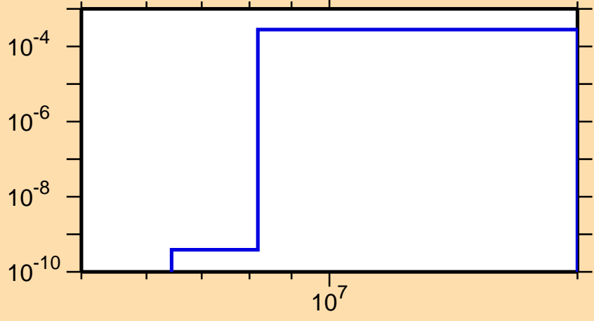
\sigma vs. E for ^{125}\text{I}(n,\alpha)
