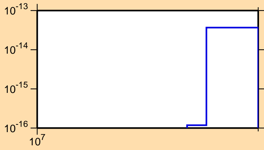
\sigma vs. E for ^{126}\text{I} (mt 34)
