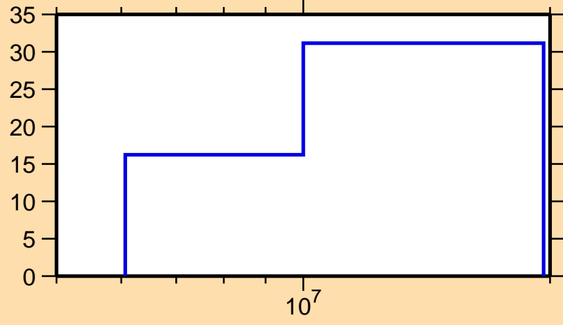
\Delta\sigma/\sigma vs. E for ^{126}\text{I}(n,\text{inel.})
