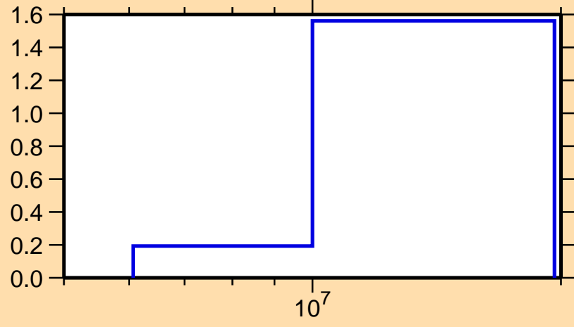
\sigma vs. E for ^{126}\text{I}(n,2n)
