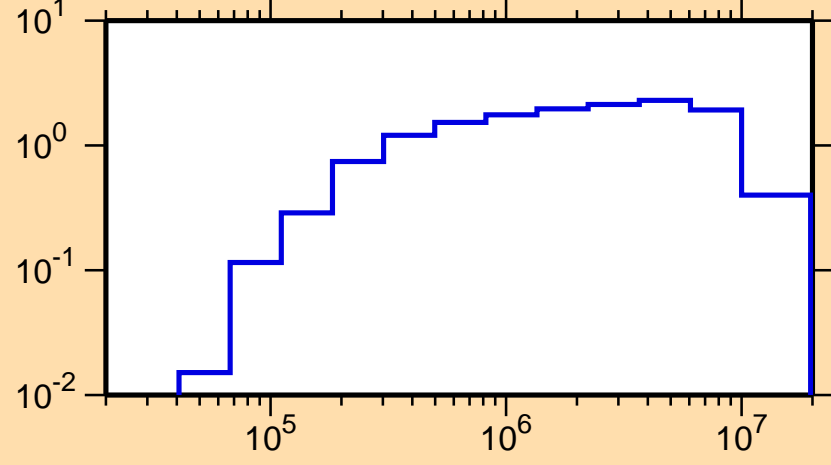
\sigma vs. E for ^{126}\text{I}(n,\text{inel.})
