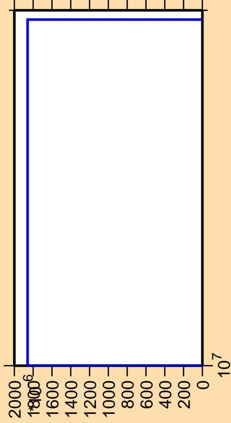
\Delta\sigma/\sigma vs. E for ^{126}\text{I} (mt 34)
