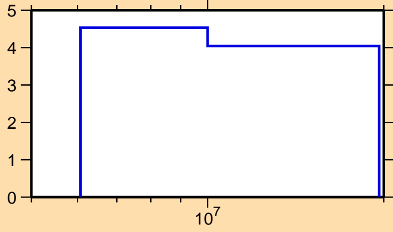
\Delta\sigma/\sigma vs. E for ^{126}\text{I}(n,\text{tot.})
