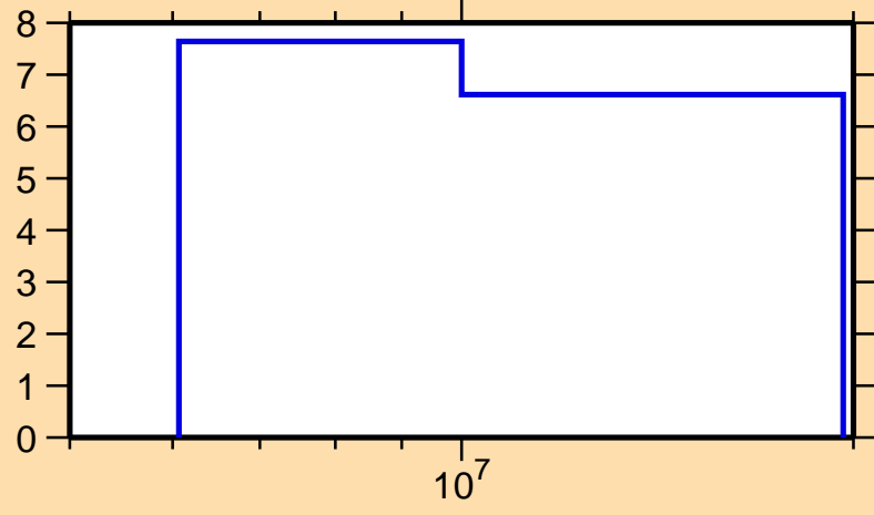
\Delta\sigma/\sigma vs. E for ^{126}\text{I}(n,\text{nonel.})
