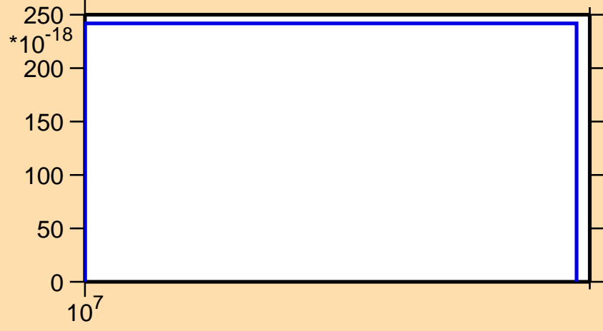
\sigma vs. E for ^{126}\text{I} (mt 34)
