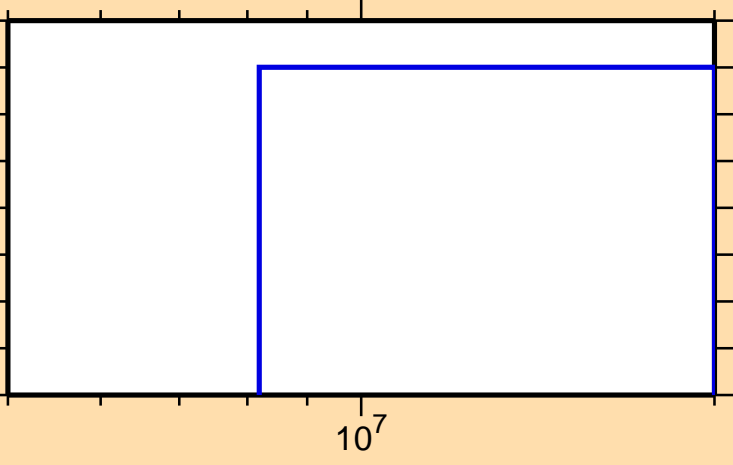
\sigma vs. E for ^{126}\text{I}(n,\text{He3})
