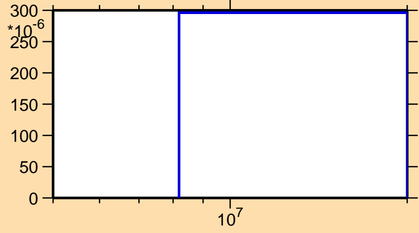
\sigma vs. E for ^{126}\text{I}(n,3n)
