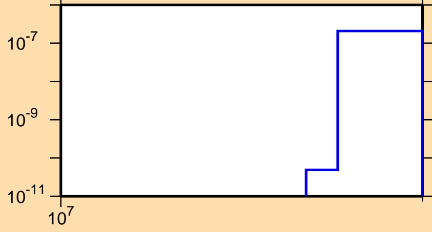
\sigma vs. E for ^{128}\text{I}(n,nt)
