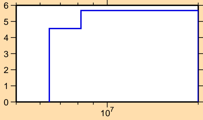
\Delta\sigma/\sigma vs. E for ^{128}\text{I}(n,\text{el.})
