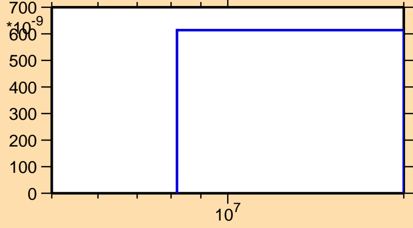
\sigma vs. E for ^{128}\text{I}(n,nd)
