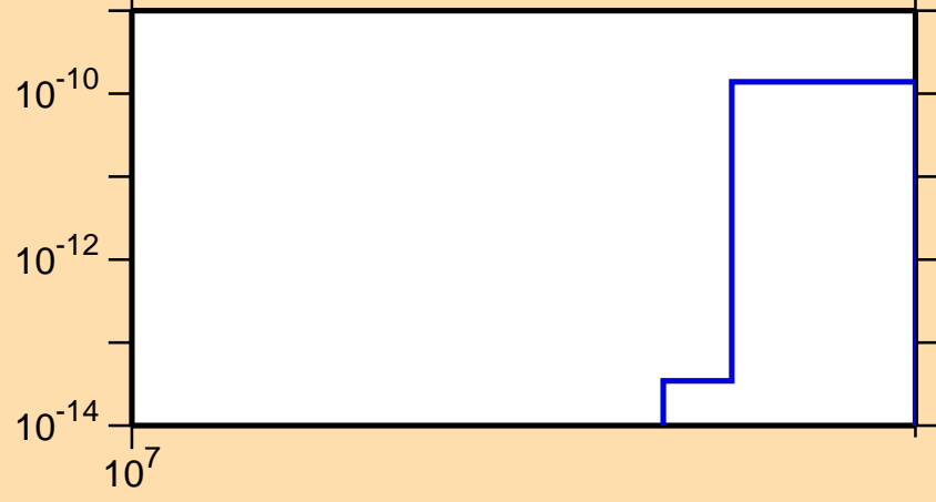
\sigma vs. E for ^{129}\text{I}(n,2n\alpha)
