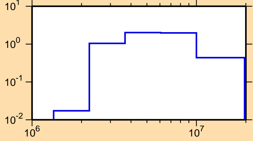
\sigma vs. E for ^{129}\text{I}(n,n\text{cont.})
