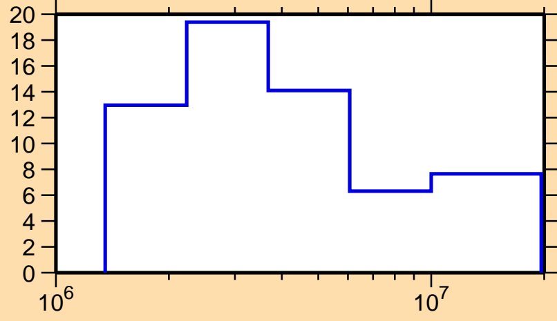
\Delta\sigma/\sigma vs. E for ^{129}\text{I}(n,el.)
