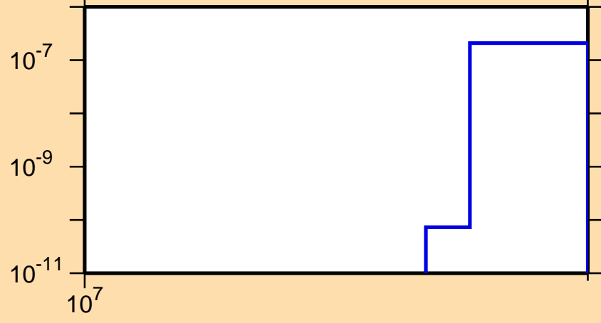
\sigma vs. E for ^{130}\text{I}(n,nt)
