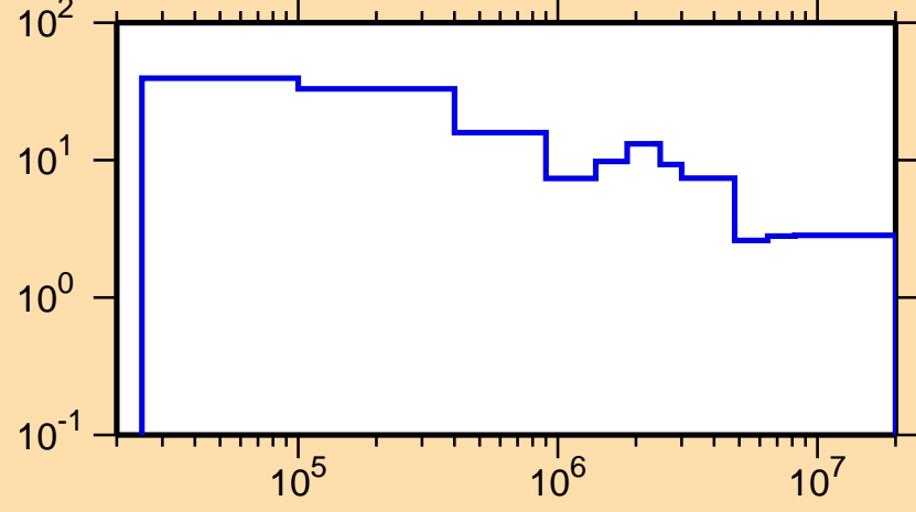
\Delta\sigma/\sigma vs. E for ^{130}\text{I}(n,\text{tot.})
