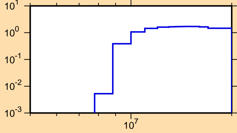
\sigma vs. E for ^{131}\text{I}(n,2n)
