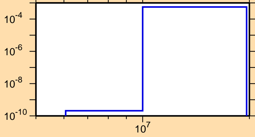
\sigma vs. E for ^{131}\text{I}(n,np)
