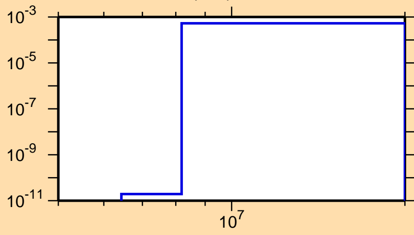
\sigma vs. E for ^{131}\text{I}(n,d)
