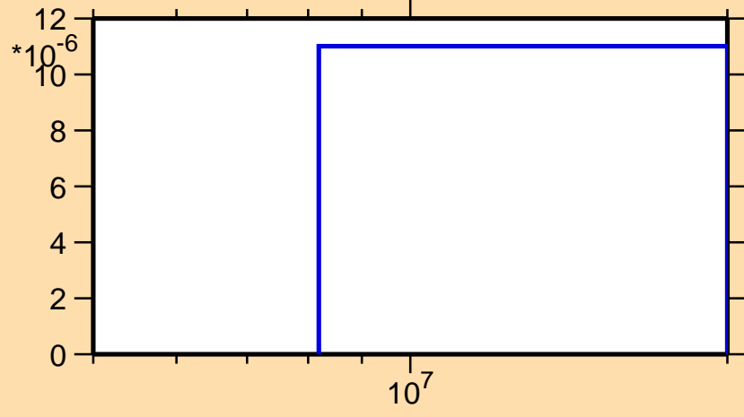
\sigma vs. E for ^{131}\text{I}(n,t)
