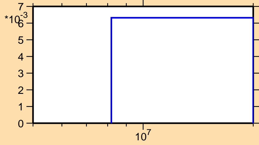
\sigma vs. E for ^{131}\text{I}(n,3n)
