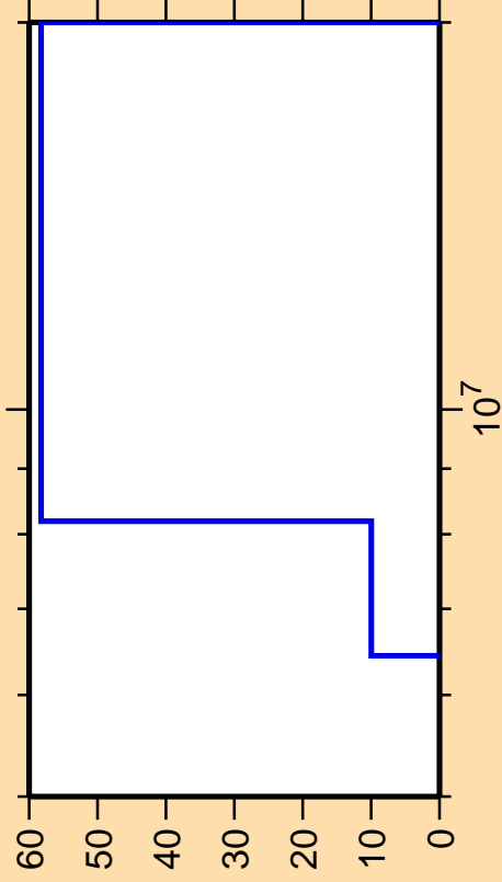
\Delta\sigma/\sigma vs. E for ^{131}\text{I}(n,d)
