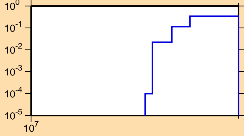
\sigma vs. E for ^{132}\text{I}(n,3n)
