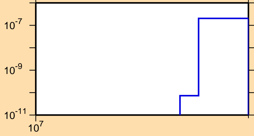
\sigma vs. E for ^{132}\text{I}(n,nt)
