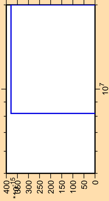
\Delta\sigma/\sigma vs. E for ^{132}\text{I} (mt 11)
