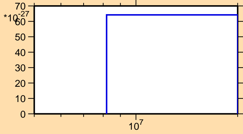
\sigma vs. E for ^{132}\text{I} (mt 11)
