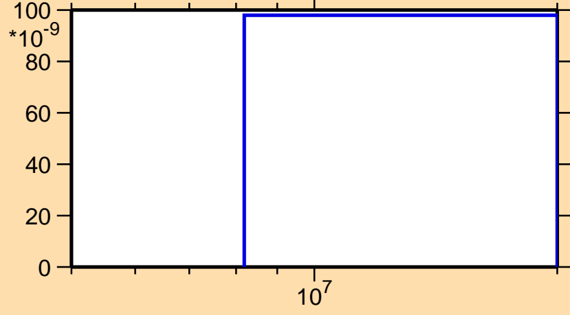
\sigma vs. E for ^{132}\text{I}(n,nd)
