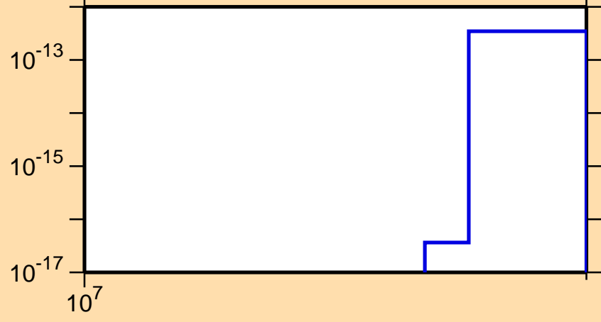
\sigma vs. E for ^{133}\text{I}(n,\text{He}3)
