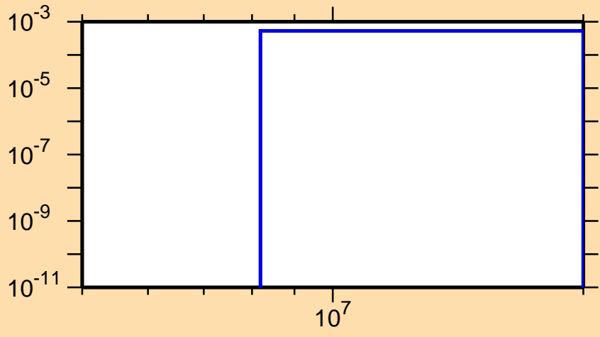
\sigma vs. E for ^{133}\text{I}(n,np)
