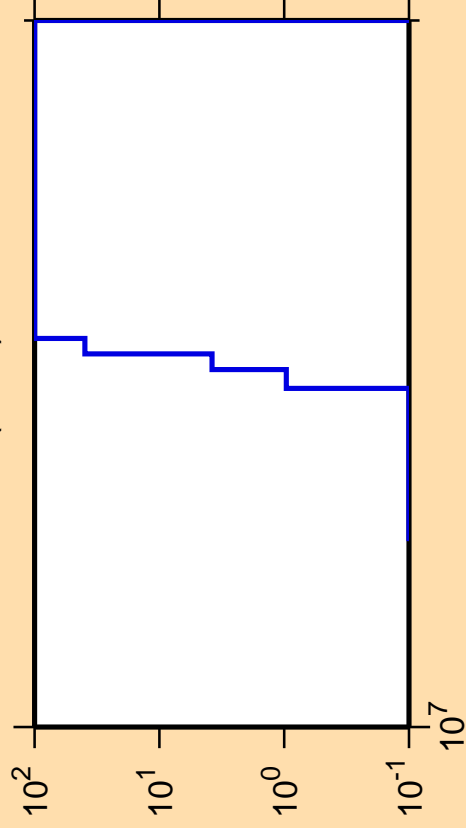
\Delta\sigma/\sigma vs. E for ^{134}\text{I}(n,nd)
