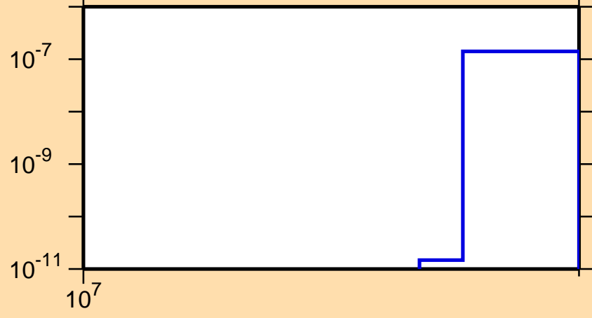
\sigma vs. E for ^{134}\text{I}(n,nt)
