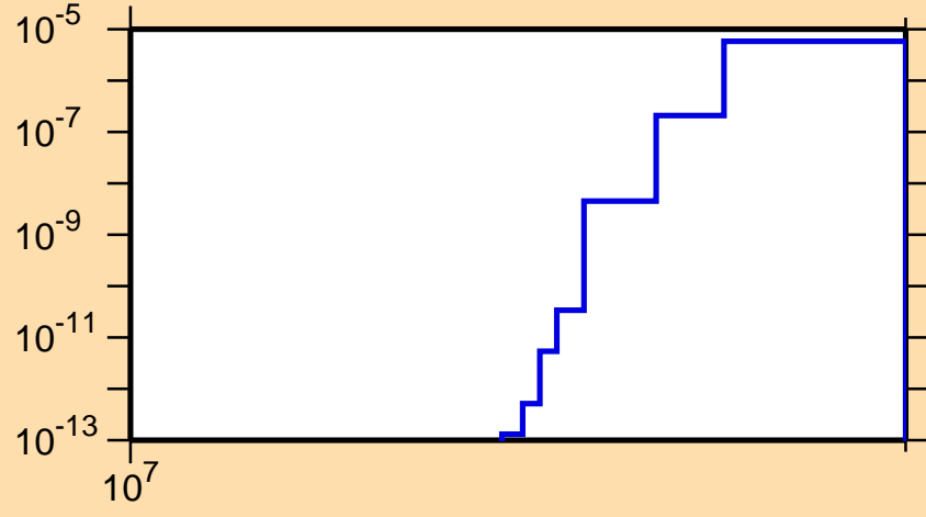
\sigma vs. E for ^{134}\text{I}(n,nd)
