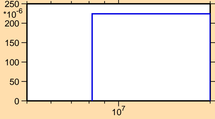
\sigma vs. E for ^{134}\text{I}(n,np)
