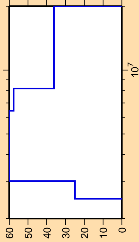
\Delta\sigma/\sigma vs. E for ^{134}\text{I}(n,p)
