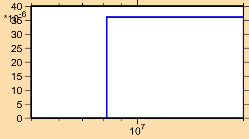
\sigma vs. E for ^{134}\text{I}(n,t)
