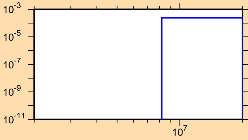
\sigma vs. E for ^{134}\text{I}(n,d)
