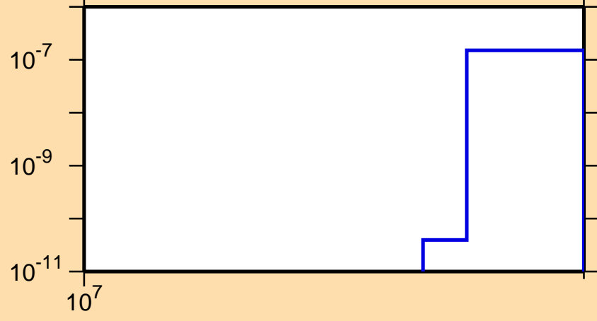
\sigma vs. E for ^{135}\text{I}(n,\text{nd})
