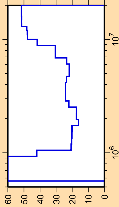
\Delta\sigma/\sigma vs. E for ^{135}\text{I}(n,\text{inel.})
