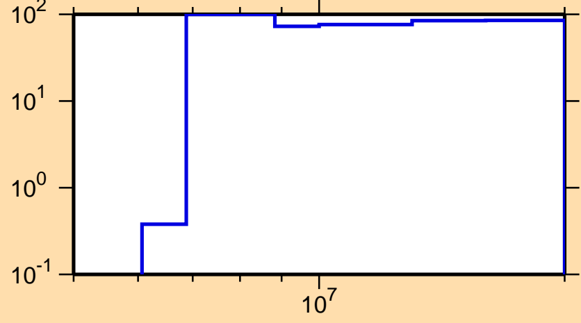
\Delta\sigma/\sigma vs. E for ^{135}\text{I}(n,p)
