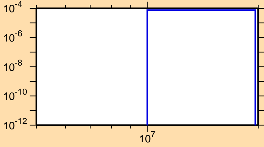
\sigma vs. E for ^{135}\text{I}(n,np)
