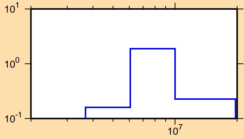
\sigma vs. E for ^{135}\text{I}(n,n\text{cont.})
