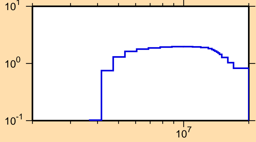
\sigma vs. E for ^{136}\text{I}(n,2n)
