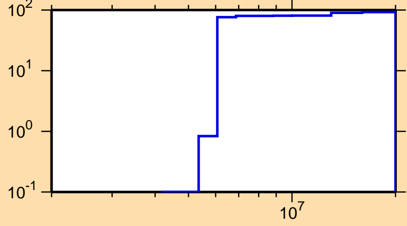
\Delta\sigma/\sigma vs. E for ^{136}\text{I}(n,p)
