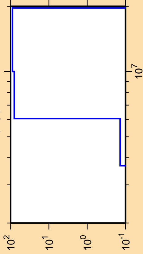
\Delta\sigma/\sigma vs. E for ^{136}\text{I}(n,p)
