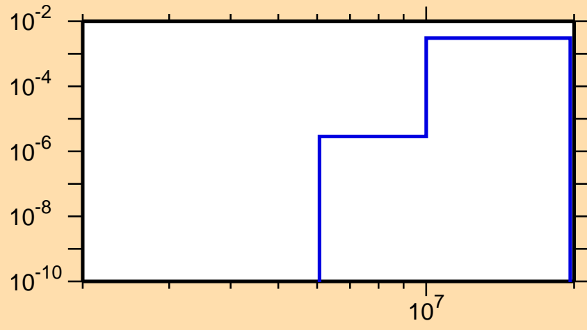
\sigma vs. E for ^{136}\text{I}(n,p)
