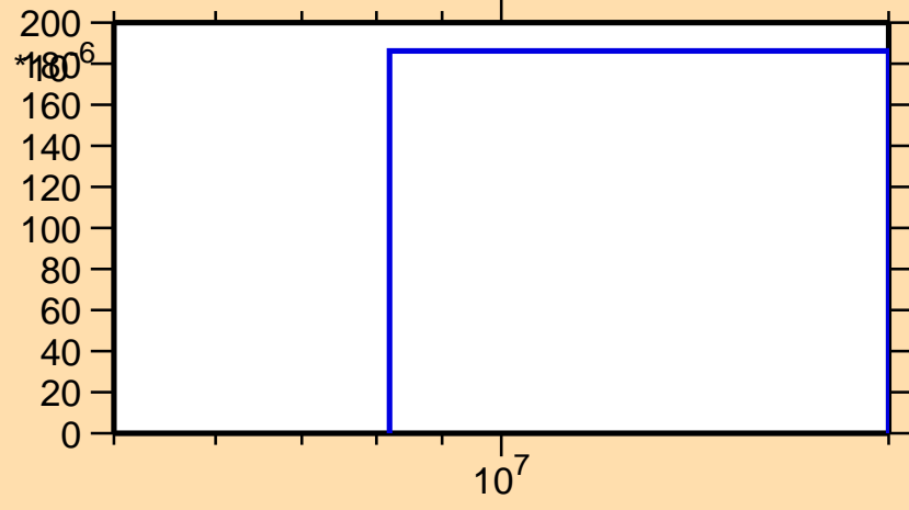
\sigma vs. E for ^{136}\text{I}(n,d)
