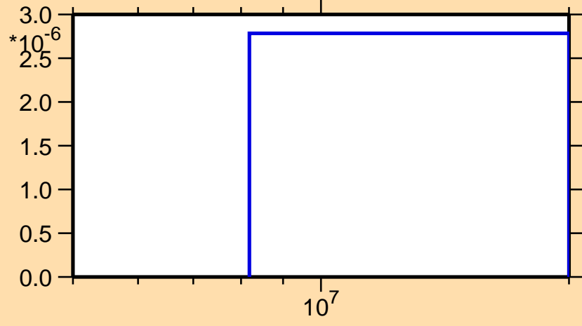
\sigma vs. E for ^{136}\text{I}(n,nd)
