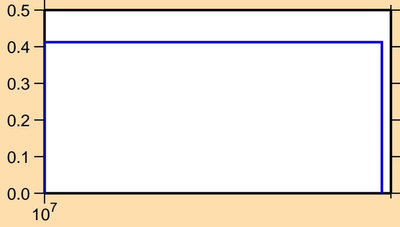
\sigma vs. E for ^{136}\text{I}(n,3n)
