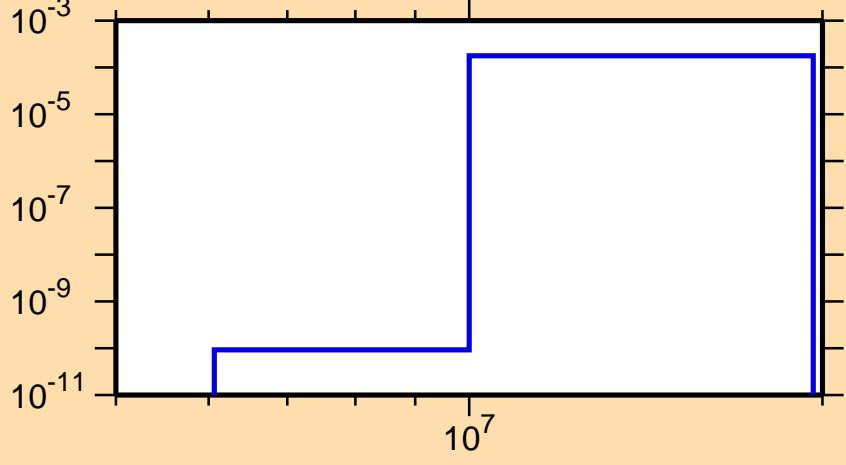
\sigma vs. E for ^{136}\text{I}(n,n\alpha)
