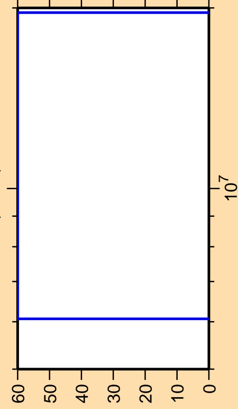
\Delta\sigma/\sigma vs. E for ^{136}\text{I}(n,n\alpha)
