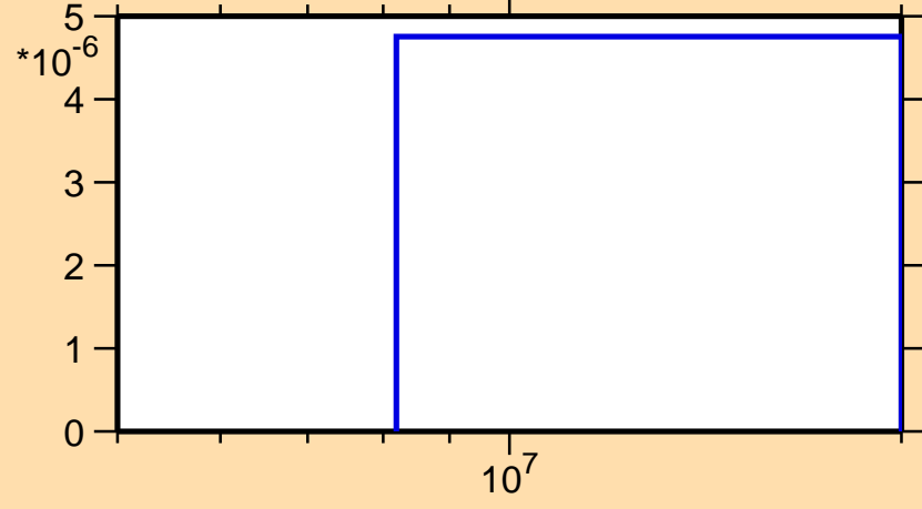
\sigma vs. E for ^{136}\text{I}(n,nd)
