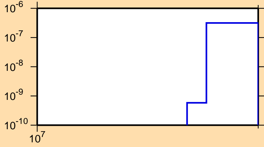
\sigma vs. E for ^{137}\text{I}(n,2np)
