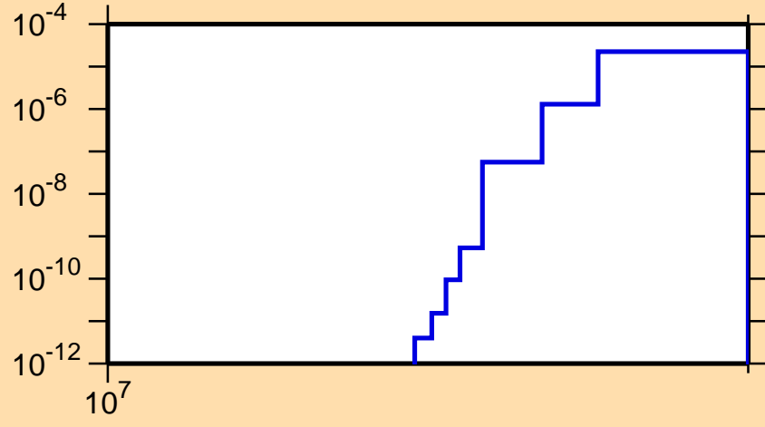
\sigma vs. E for ^{137}\text{I}(n,nd)
