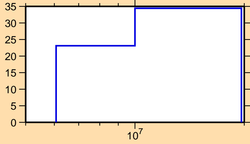
\Delta\sigma/\sigma vs. E for ^{137}\text{I}(n,el.)
